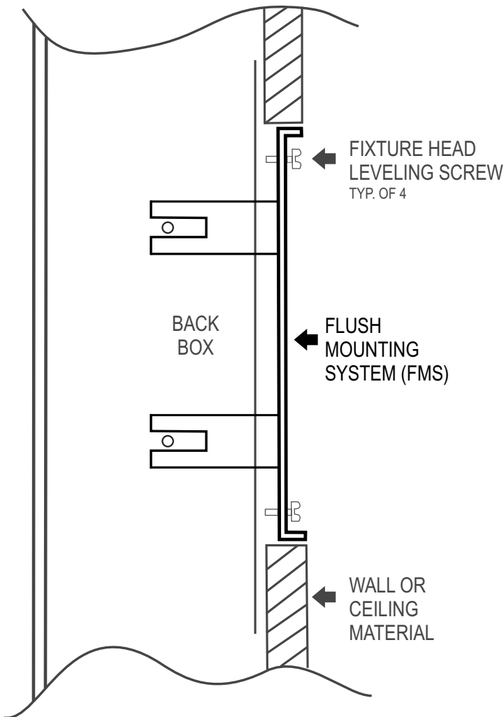
SIDE FLUSH VIEW
