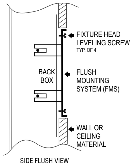
SIDE FLUSH VIEW
